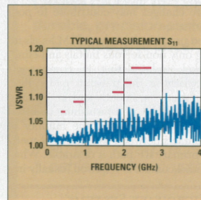
▲ Fig. 2 Typical VSWR measurement graph.
